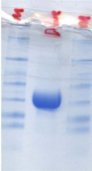
hwt 02-12-08 fluorescence
