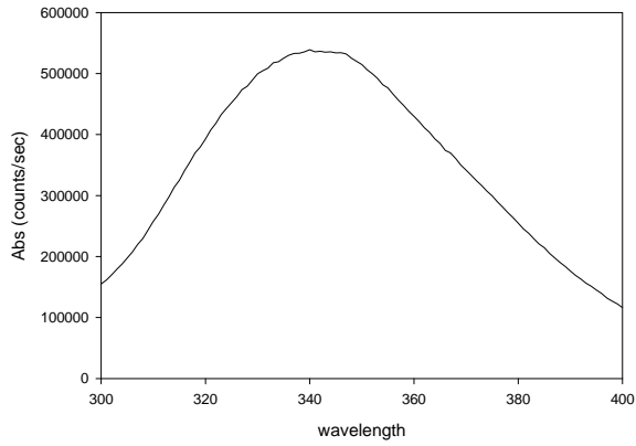
hwt 02-12-08 tmelt
