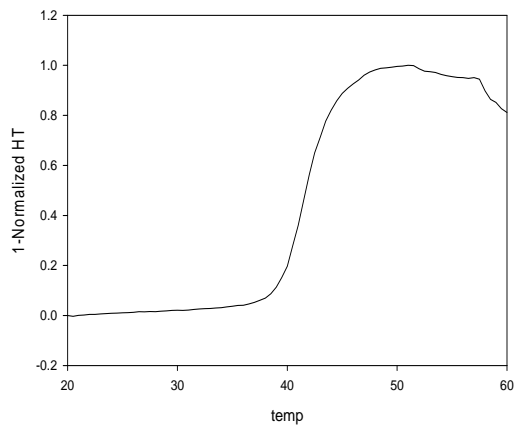
hwt 02-12-08 tmelt
