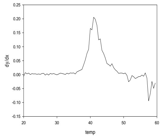
hwt 02-12-08 1st derivative of tmelt
