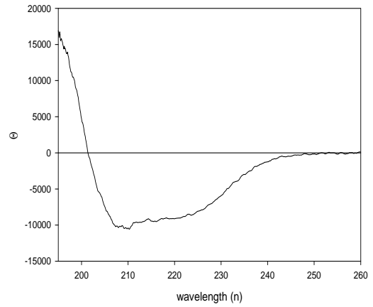
hwt 02-12-08 mwpr molar ellipticity
