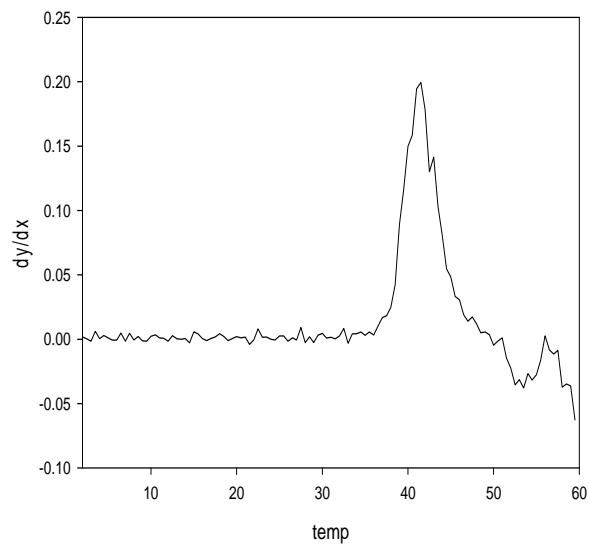
06-05-07 hwt 1st derivative of tmelt
