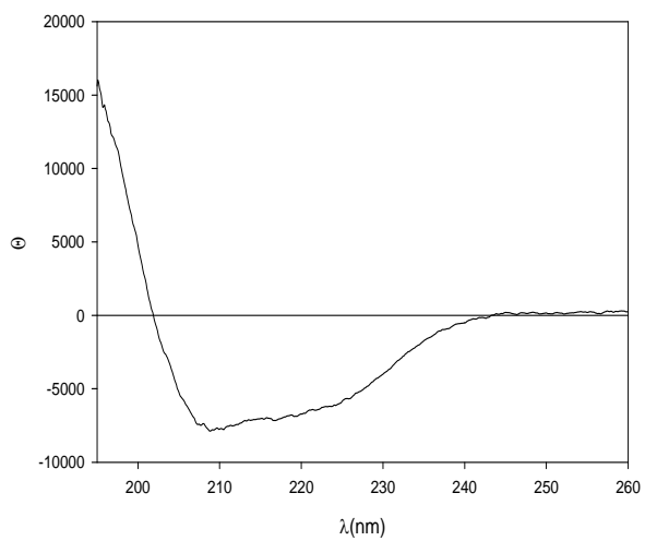
06-05-07 hwt mwpr molar ellipticity
