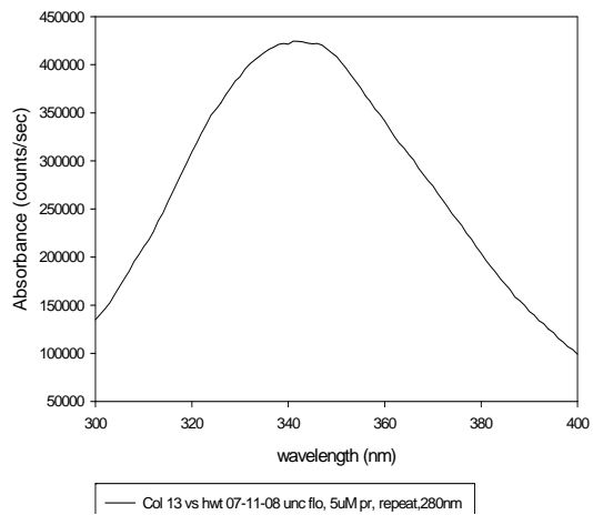
hwt 07-11-08 fluorescence
