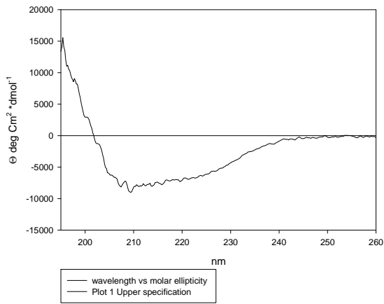
071206 hWT NBD1 Mean Residue Molar Ellipticity
