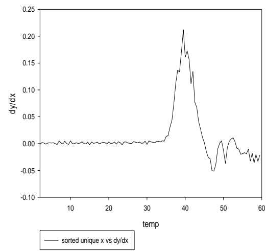
hNBD1WT110807 1st derivative of tmelt
