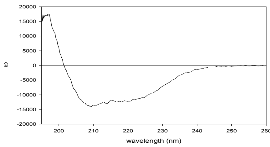
mDF 09-11-07 mwpr molar ellipticity
