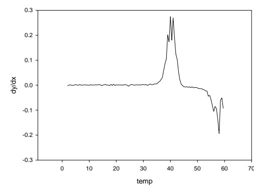
mDF 09-11-07 1st Derivative of Tmelt
