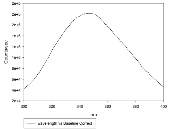
Fluorescence of m \Delta F NBD1 091406
