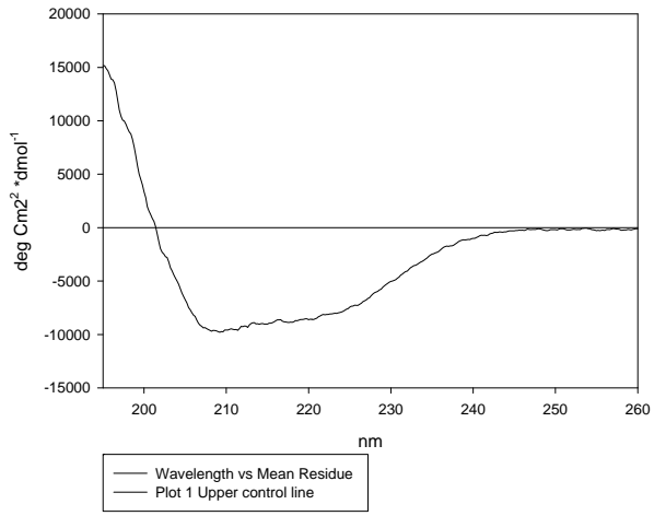
mDF NBD1 Mean Residue Molar Ellipticity
